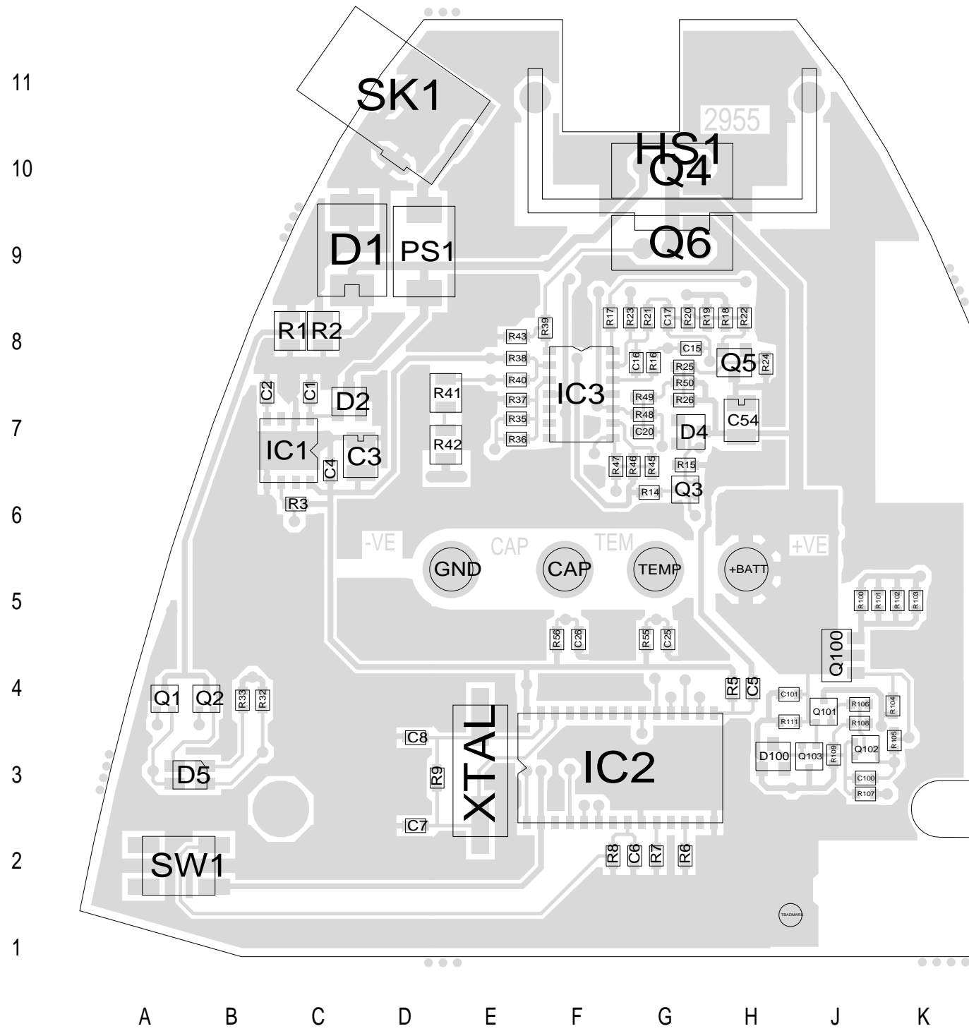
220-01411-01 TOP COPPER
