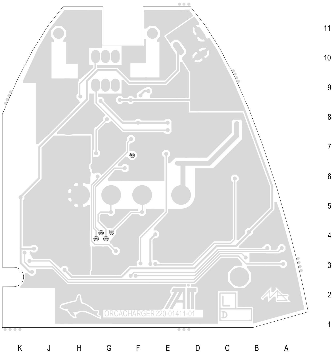
220-01411-01 BOTTOM COPPER
